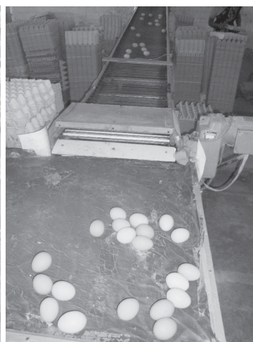
Automatic egg collection equipment
