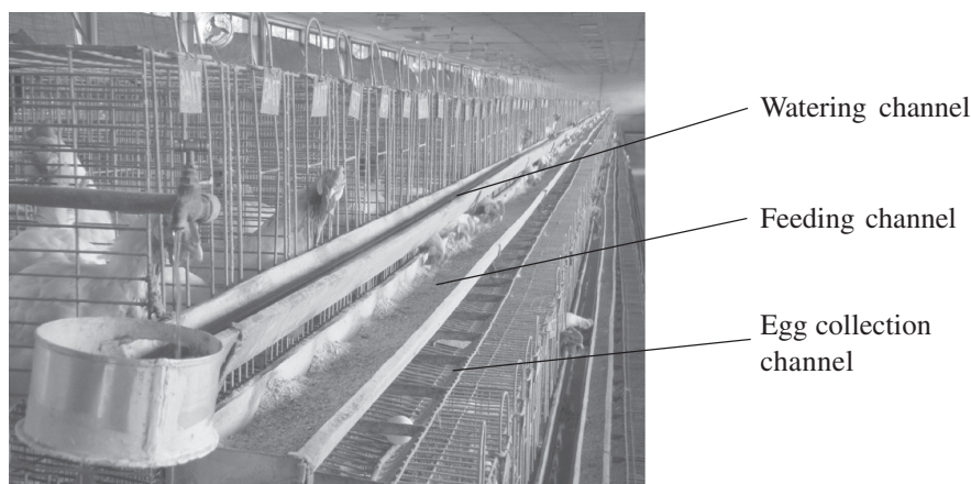
Fig. 5.12: Cage with feeding, watering and egg collection channels
