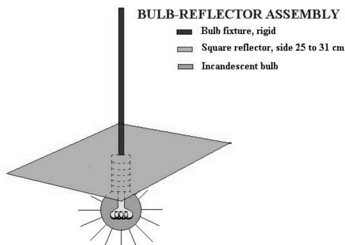
Fig. 8.3: Bulb-reflector assembly
